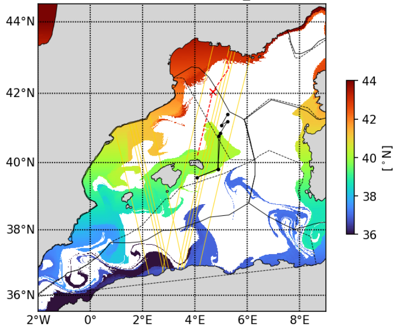
20230517 Latfrombathy_500m
