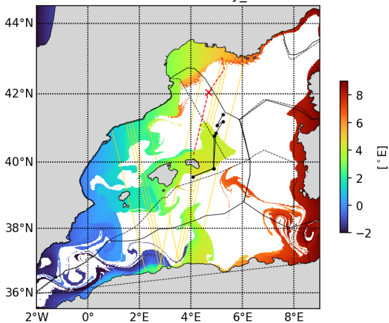
20230517 Lonfrombathy_500m
