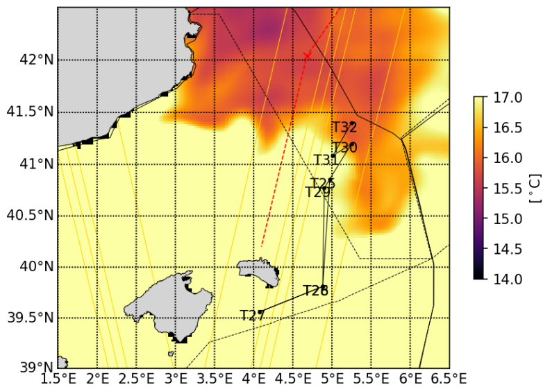
20230517 Tracer advection
