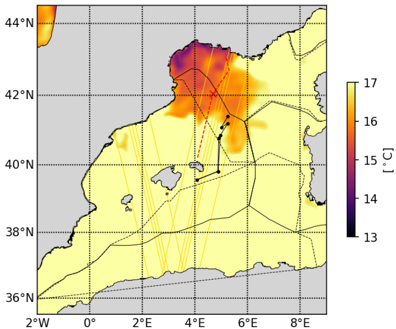
20230517 Tracer advection
