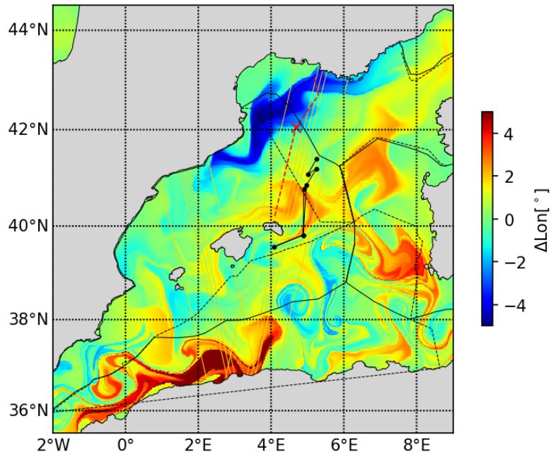
20230517 LonAdv
