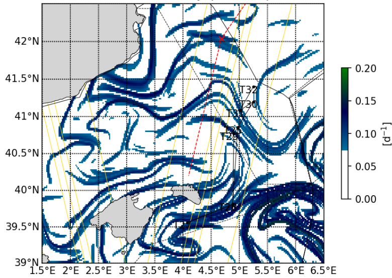
20230517 Finite Time Lyapunov Exponent
