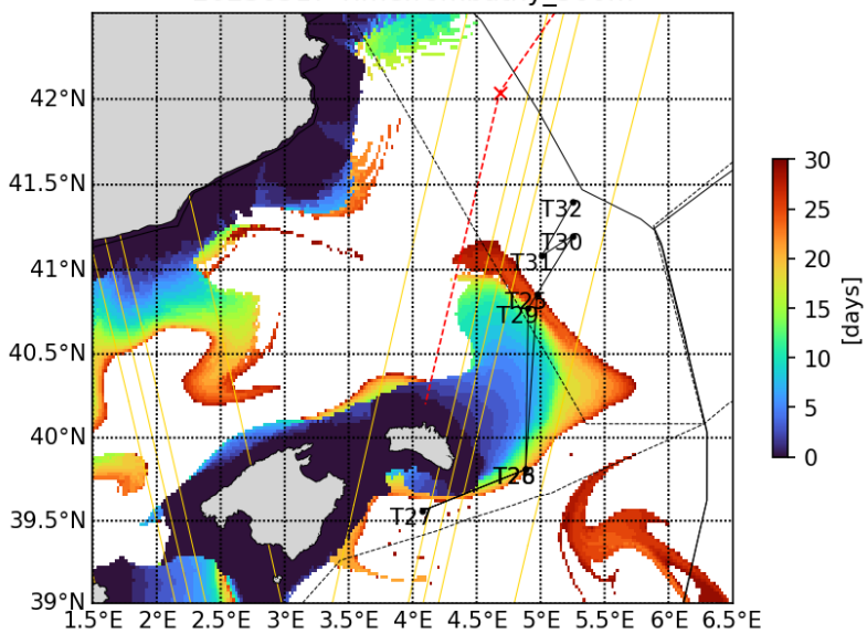
20230517 Timefrombathy_500m
