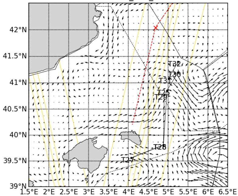
20230511_CLS_PHY
