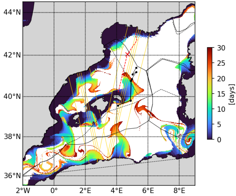
20230517 Timefrombathy_500m
