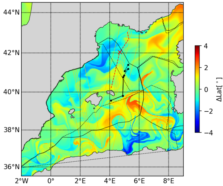
20230517 LatAdv
