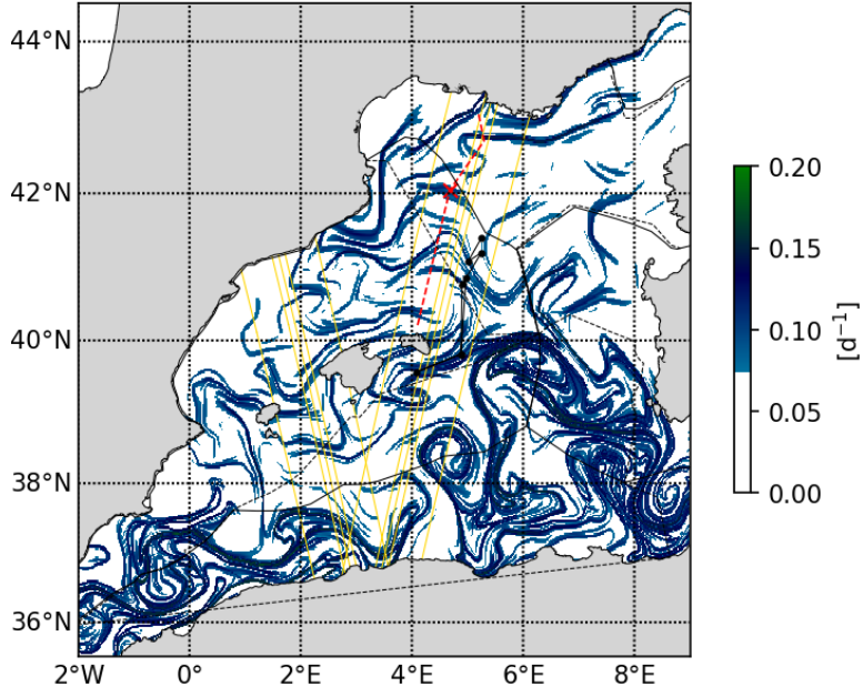
20230517 Finite Time Lyapunov Exponent
