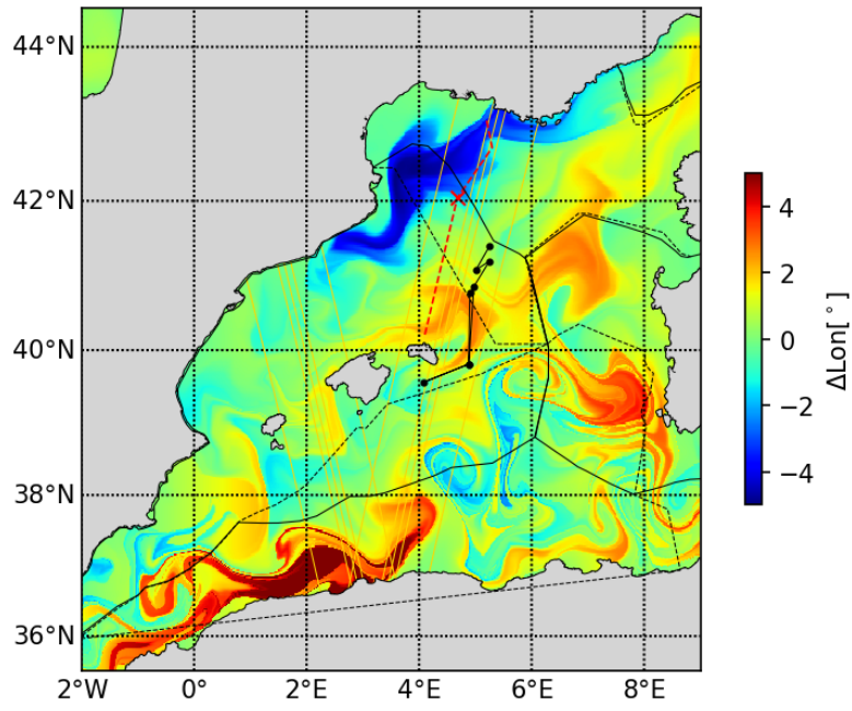
20230515 LonAdv
