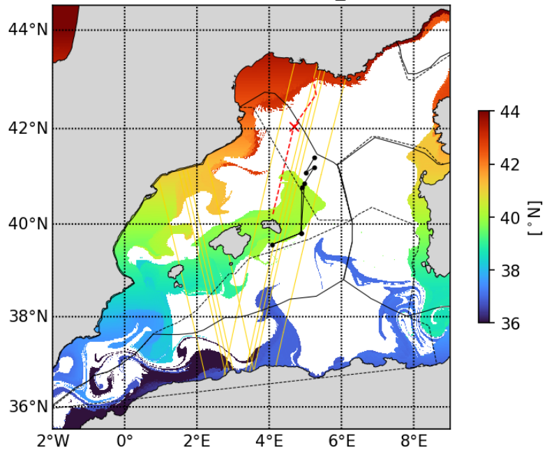
20230515 Latfrombathy_500m
