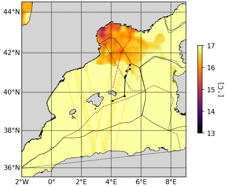
20230515 Tracer advection
