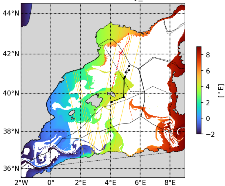
20230515 Lonfrombathy_500m
