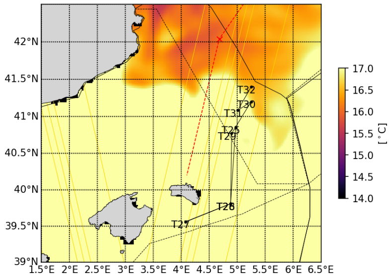
20230515 Tracer advection
