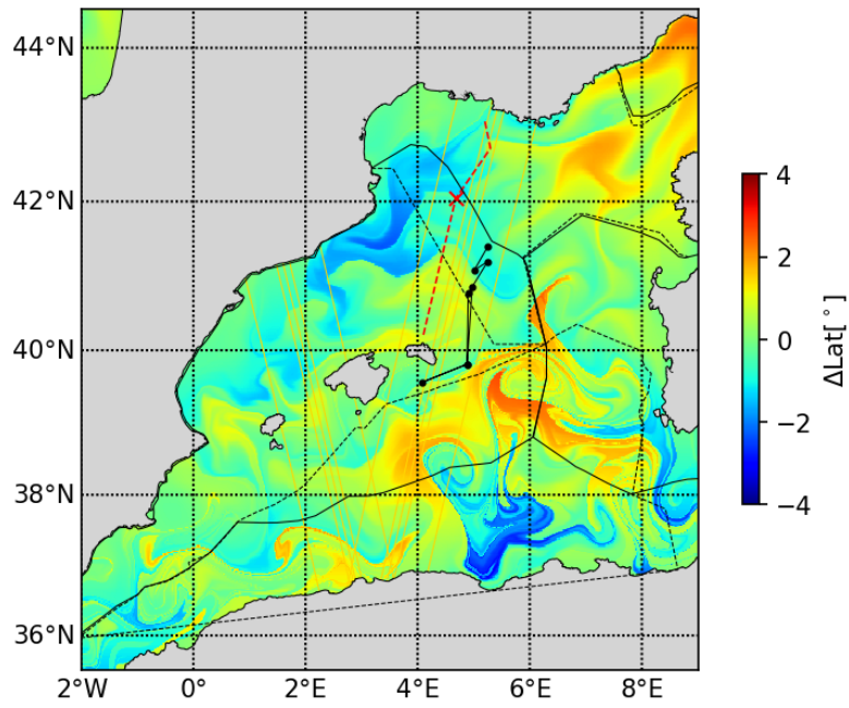
20230515 LatAdv
