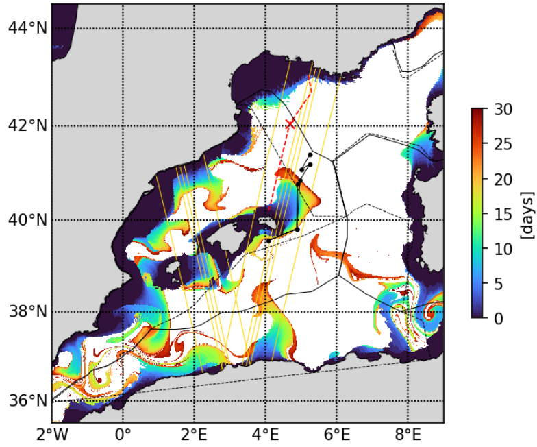
20230515 Timefrombathy_500m
