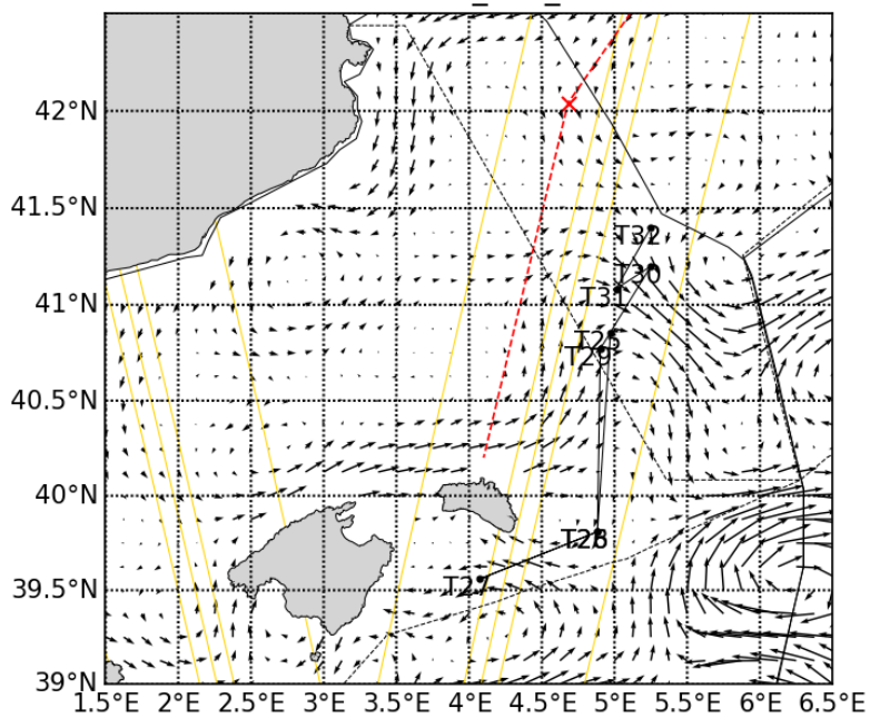
20230509_CLS_PHY
