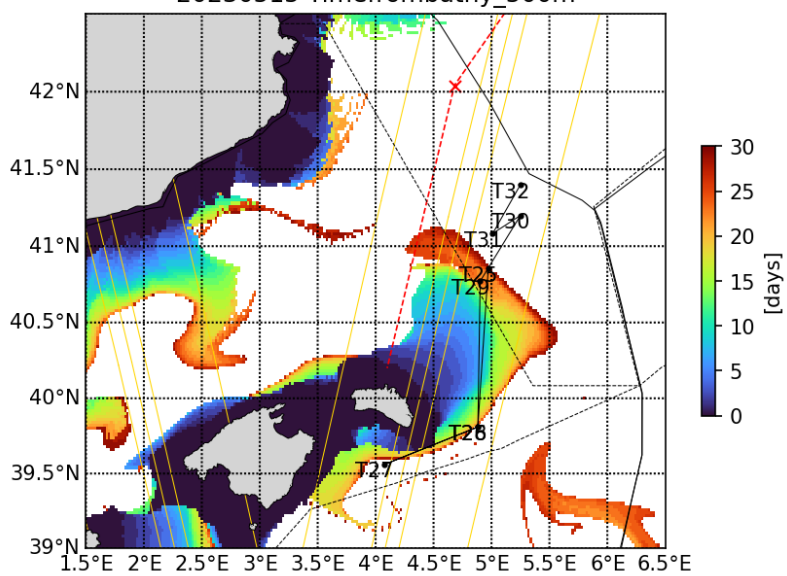
20230515 Timefrombathy_500m
