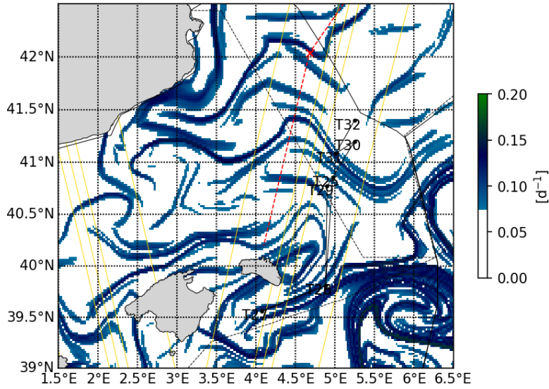
20230514 Finite Time Lyapunov Exponent
