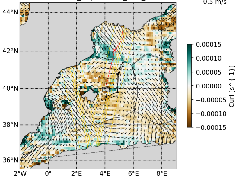
2023041016_Copernicus_PHY_WIND
