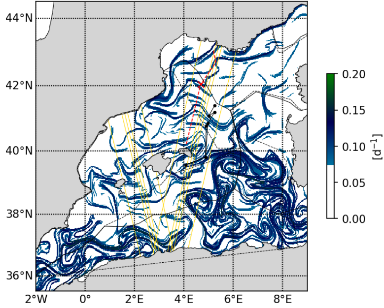
20230514 Finite Time Lyapunov Exponent
