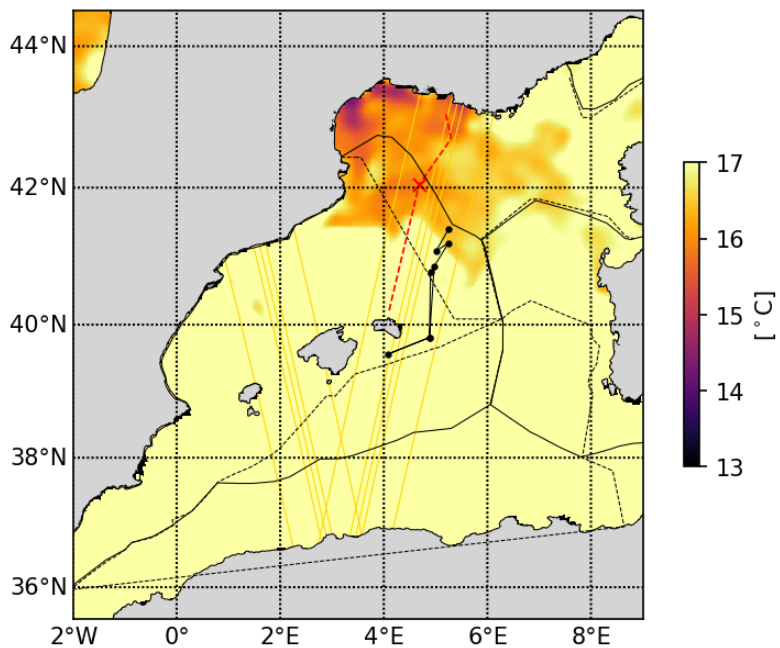
20230514 Tracer advection
