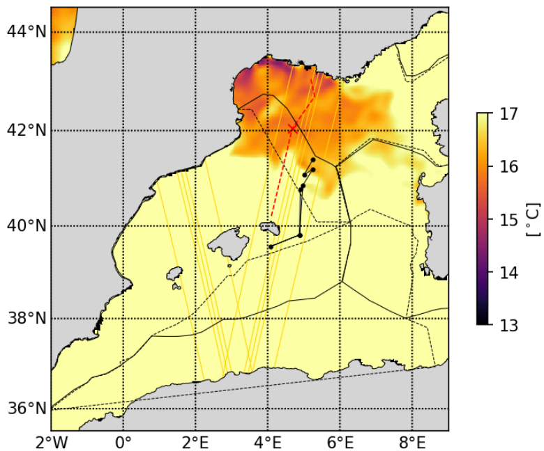
20230512 Tracer advection
