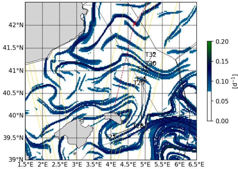
20230512 Finite Time Lyapunov Exponent
