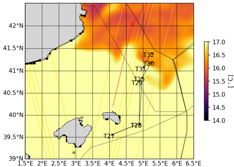
20230512 Tracer advection
