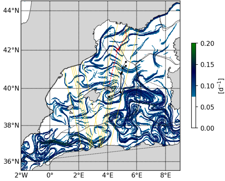
20230512 Finite Time Lyapunov Exponent
