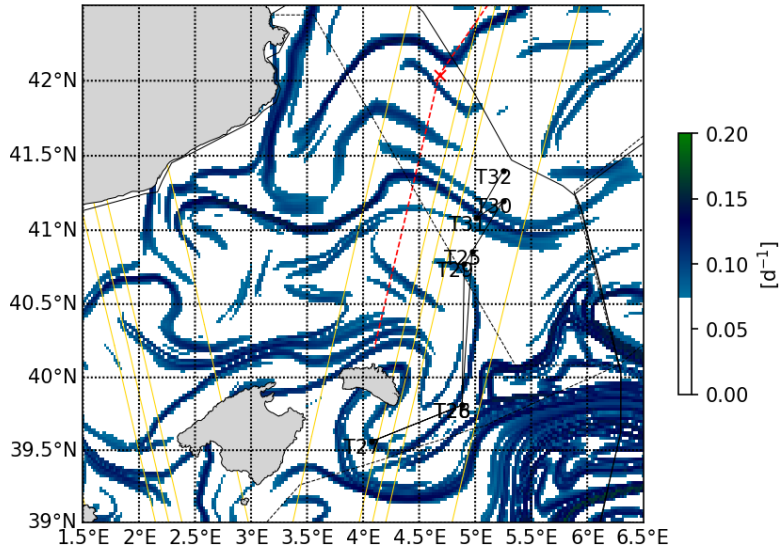
20230510 Finite Time Lyapunov Exponent
