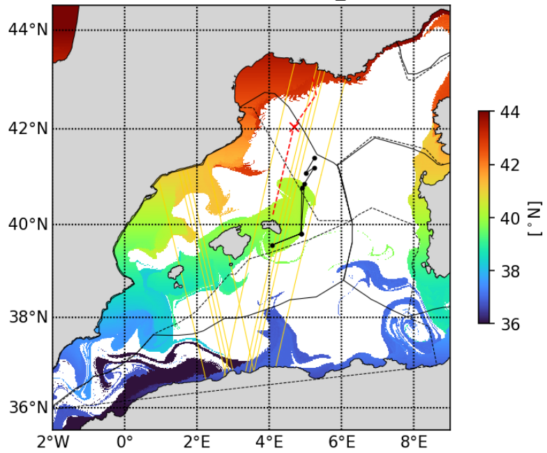
20230510 Latfrombathy_500m
