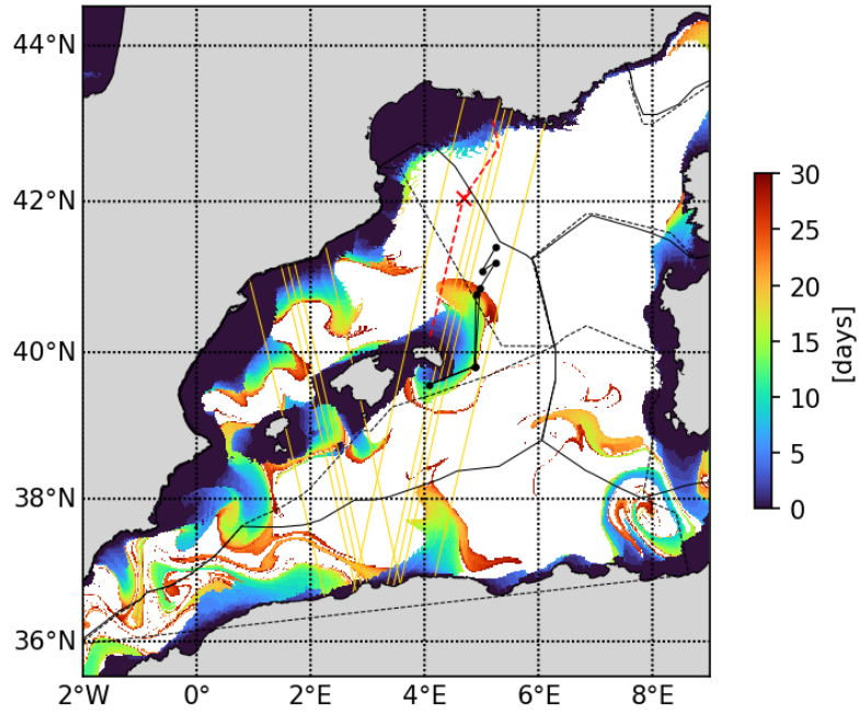
20230510 Timefrombathy_500m
