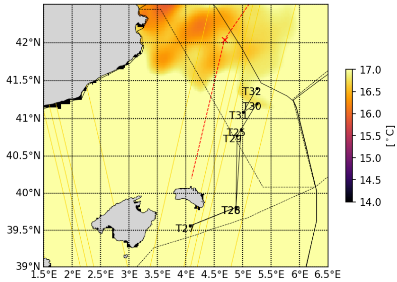
20230510 Tracer advection
