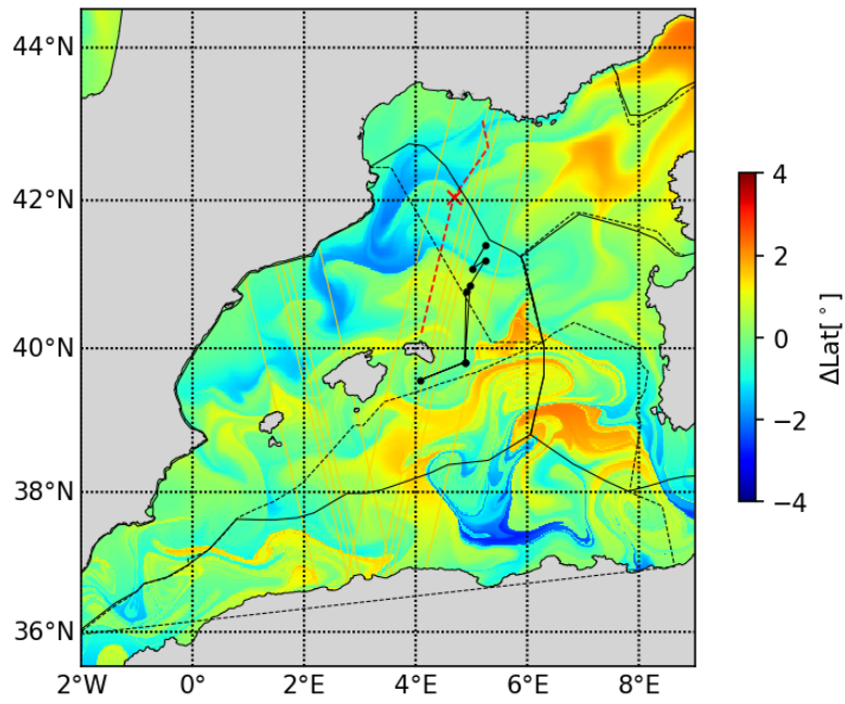
20230510 LatAdv
