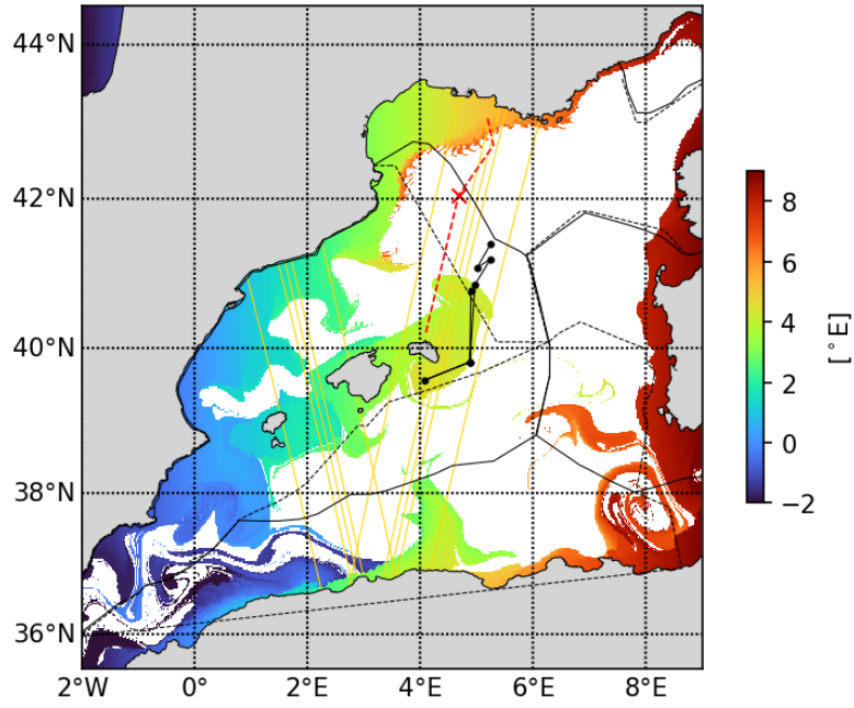
20230510 Lonfrombathy_500m
