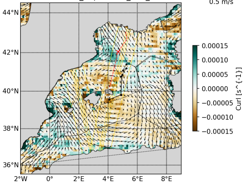
2023041017_Copernicus_PHY_WIND
