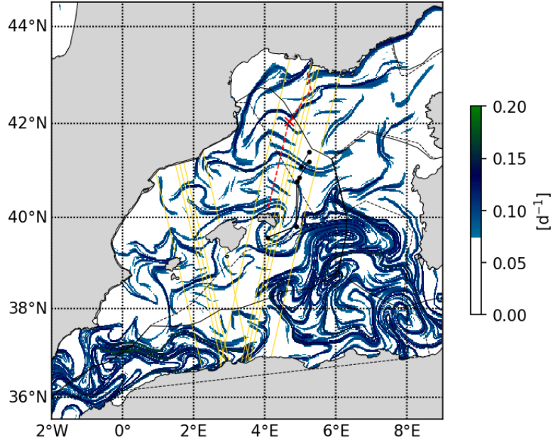
20230510 Finite Time Lyapunov Exponent
