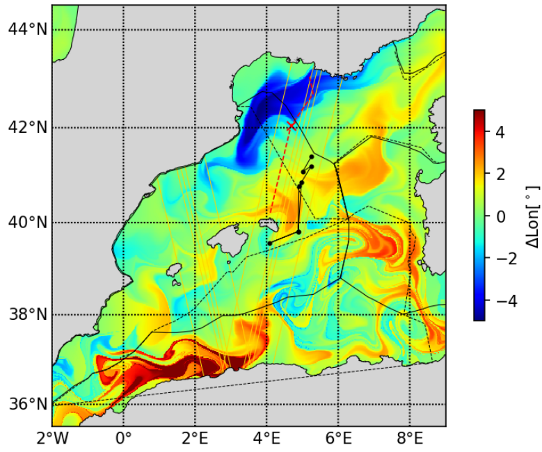
20230510 LonAdv
