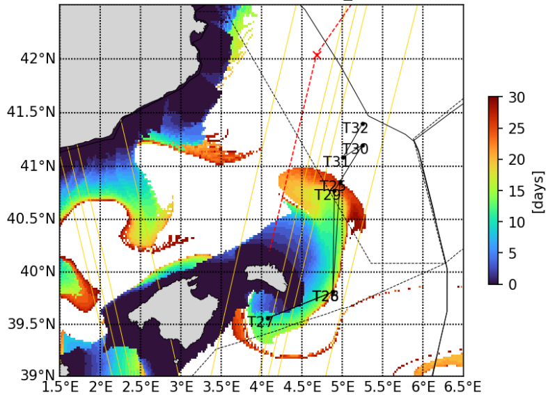
20230510 Timefrombathy_500m
