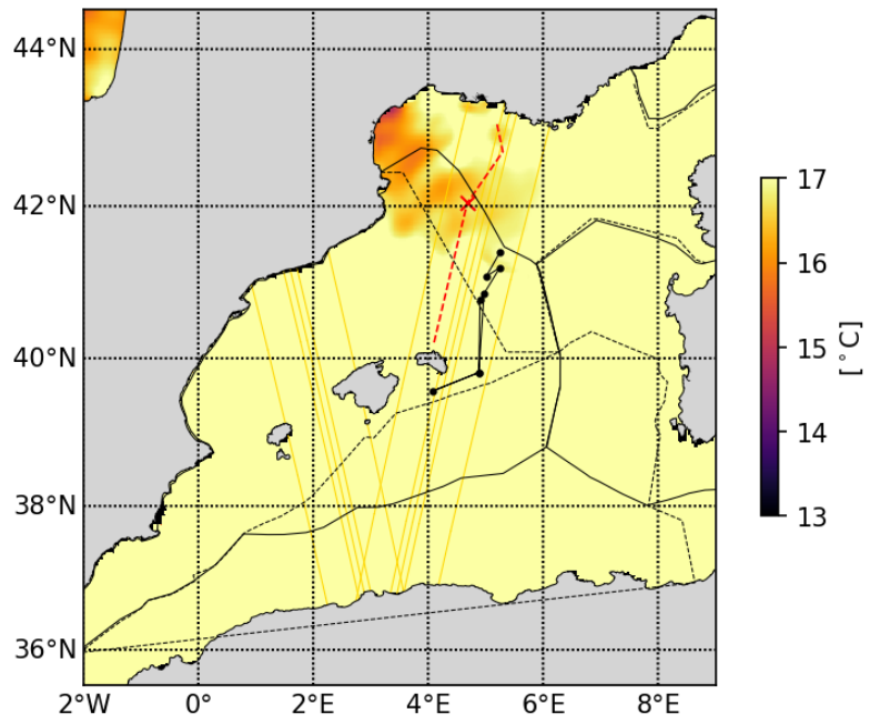
20230510 Tracer advection
