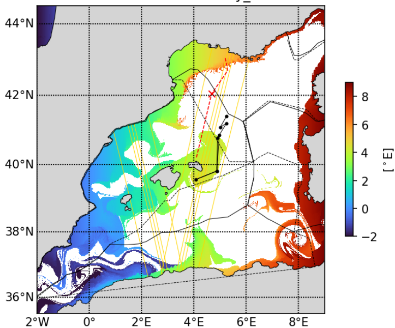
20230509 Lonfrombathy_500m
