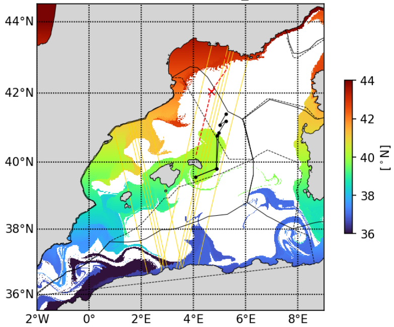
20230509 Latfrombathy_500m
