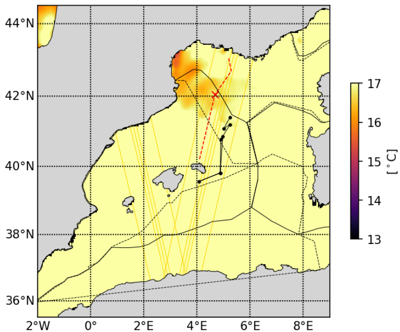
20230509 Tracer advection
