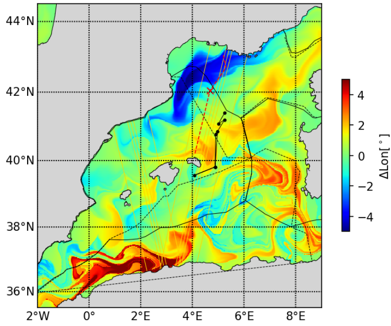
20230509 LonAdv
