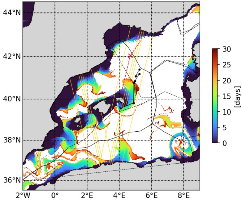
20230509 Timefrombathy_500m
