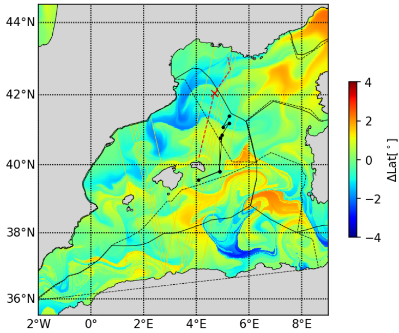
20230509 LatAdv
