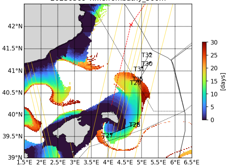
20230509 Timefrombathy_500m
