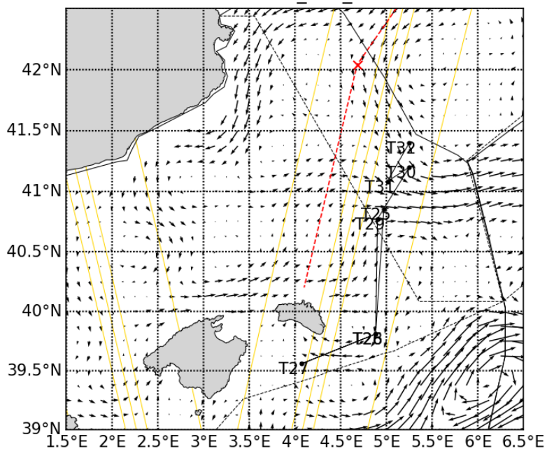
20230503_CLS_PHY
