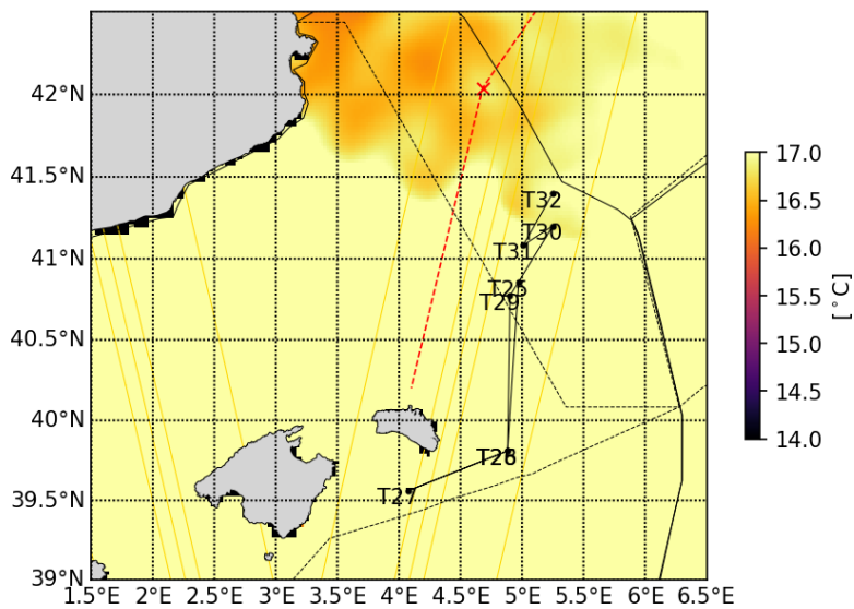
20230509 Tracer advection
