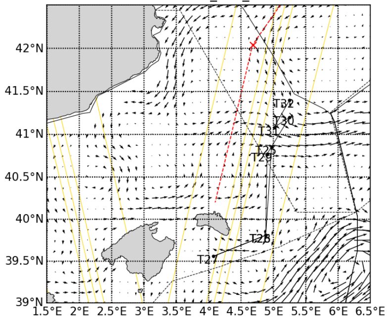
20230502_CLS_PHY
