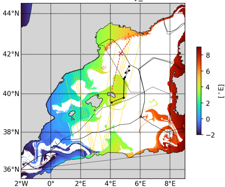
20230508 Lonfrombathy_500m
