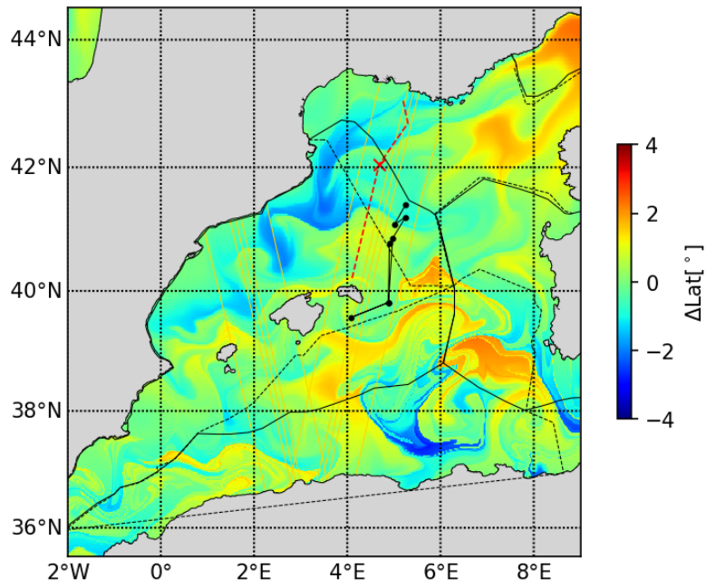
20230508 LatAdv
