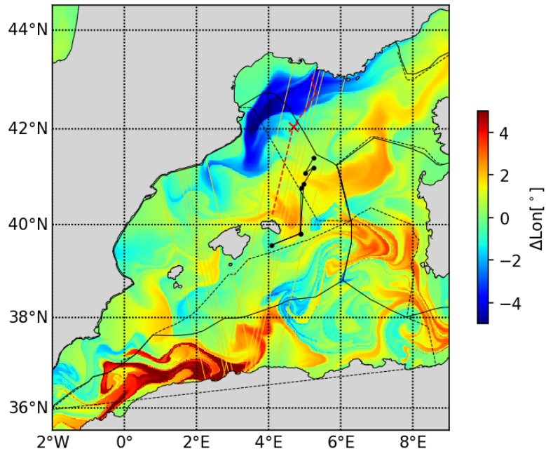
20230508 LonAdv
