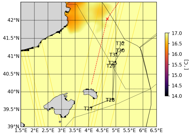
20230508 Tracer advection
