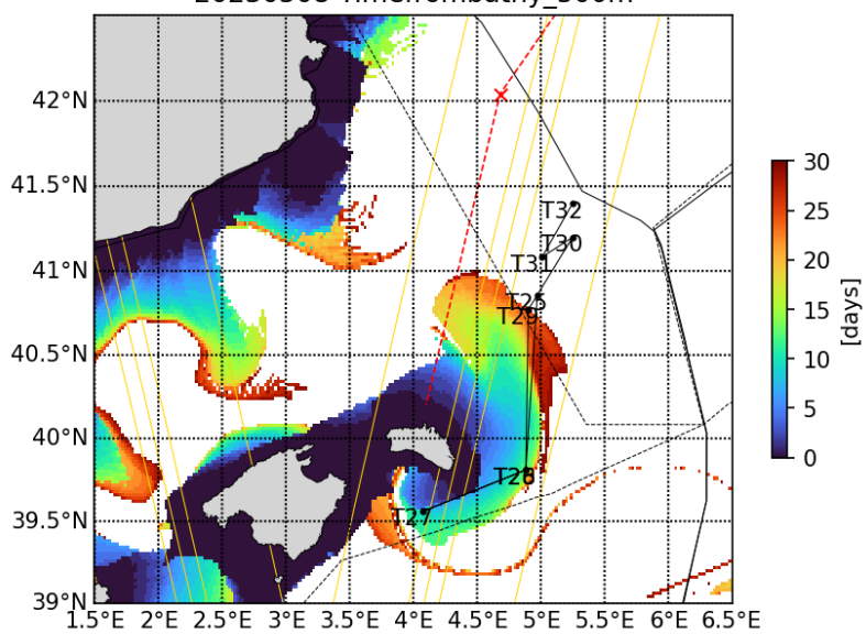
20230508 Timefrombathy_500m
