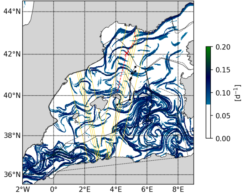
20230508 Finite Time Lyapunov Exponent
