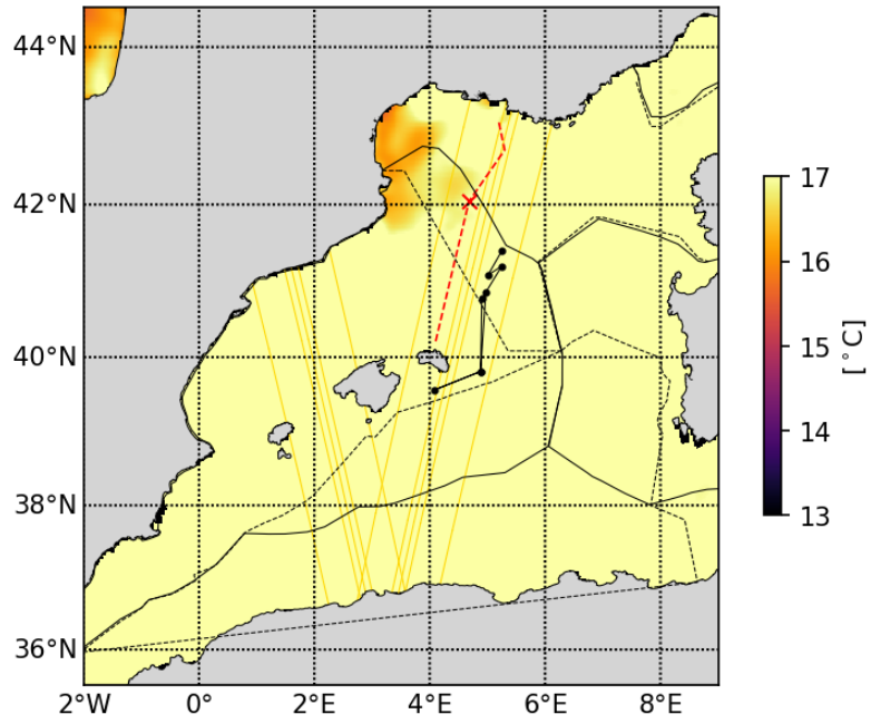
20230508 Tracer advection
