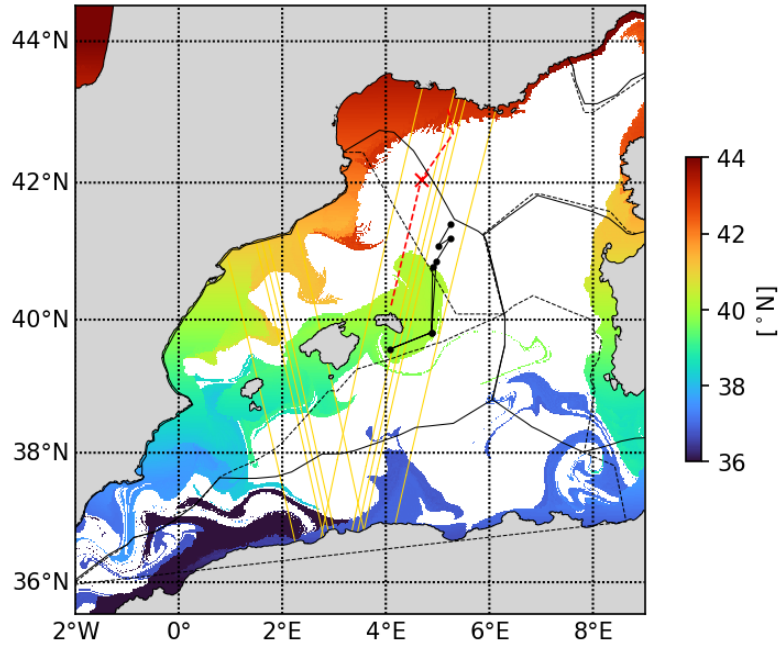
20230508 Latfrombathy_500m
