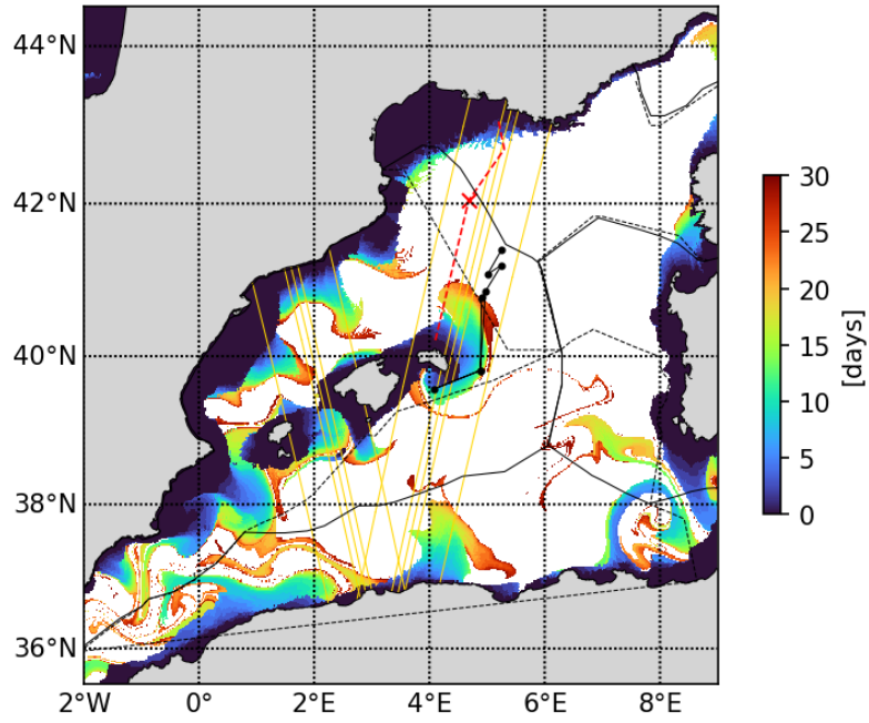
20230508 Timefrombathy_500m
