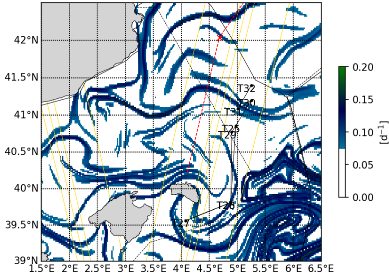
20230508 Finite Time Lyapunov Exponent
