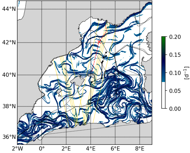
20230507 Finite Time Lyapunov Exponent
