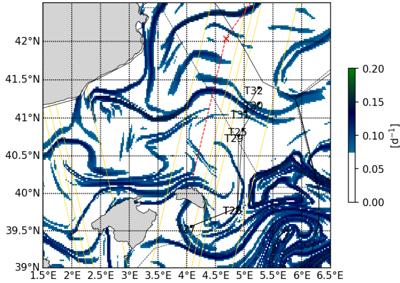
20230507 Finite Time Lyapunov Exponent
