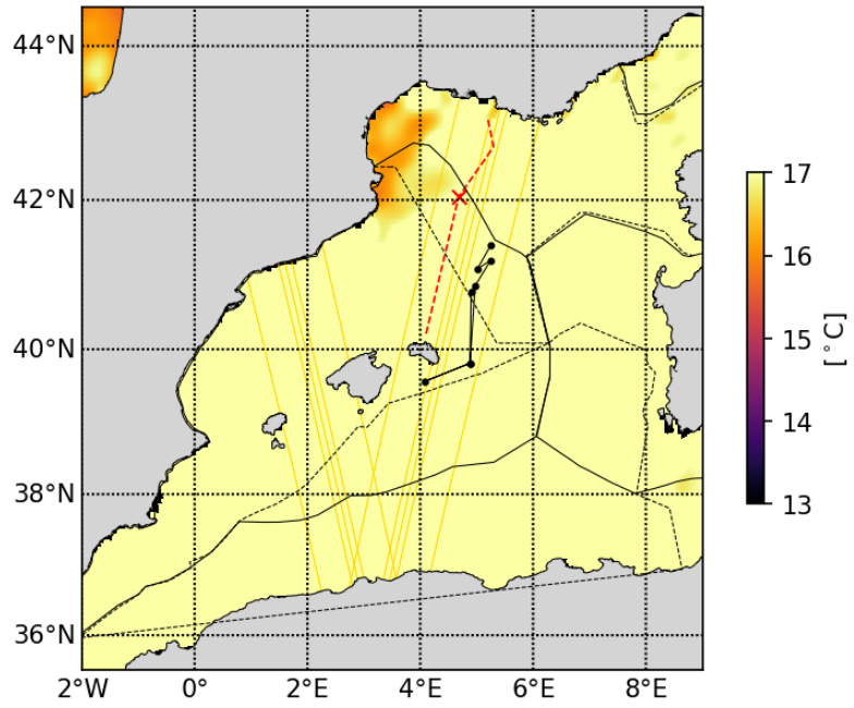
20230507 Tracer advection
