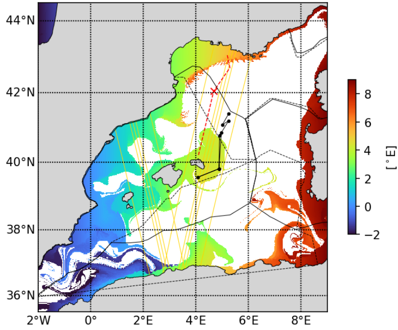
20230507 Lonfrombathy_500m
