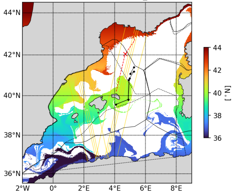
20230507 Latfrombathy_500m
