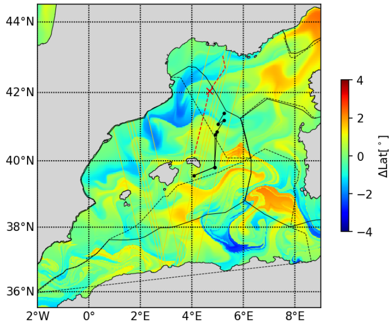
20230507 LatAdv
