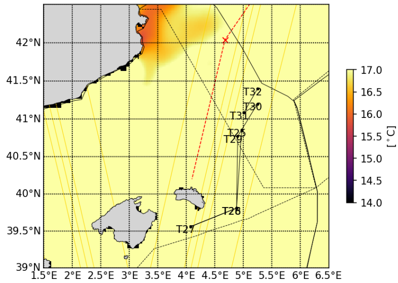
20230507 Tracer advection
