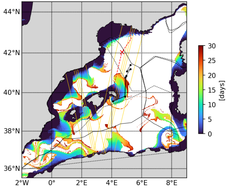
20230507 Timefrombathy_500m
