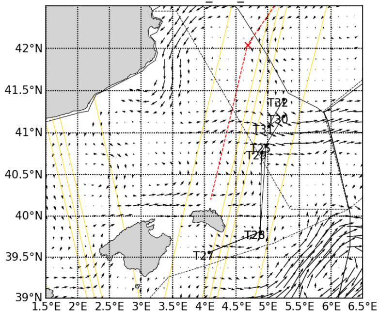
20230501_CLS_PHY
