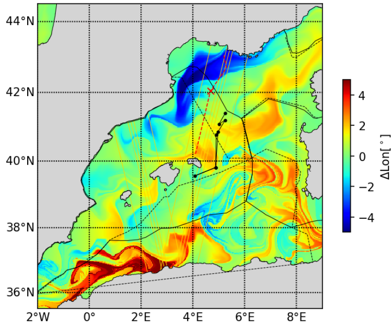
20230507 LonAdv
