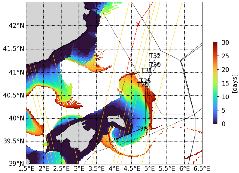
20230507 Timefrombathy_500m
