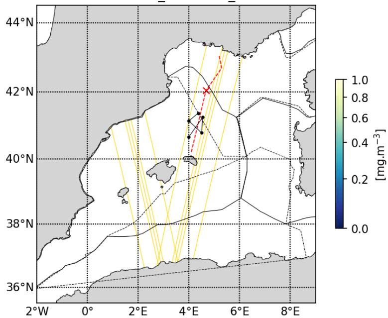
20230425_Sentinel3_CHL
