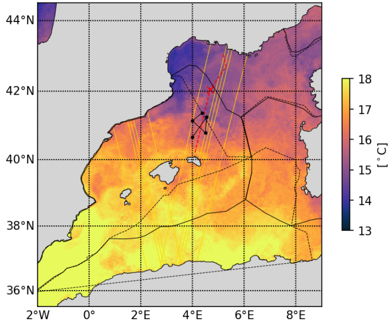
20230424_CLS_SST_5d
