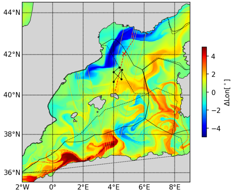
20230426 LonAdv
