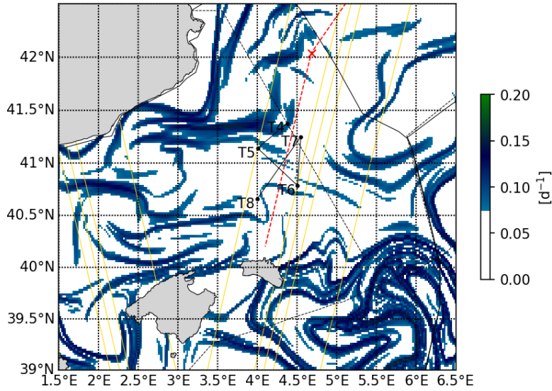
20230426 Finite Time Lyapunov Exponent
