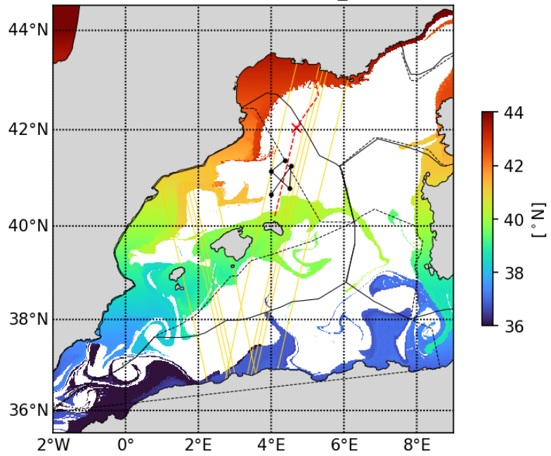
20230426 Latfrombathy_500m
