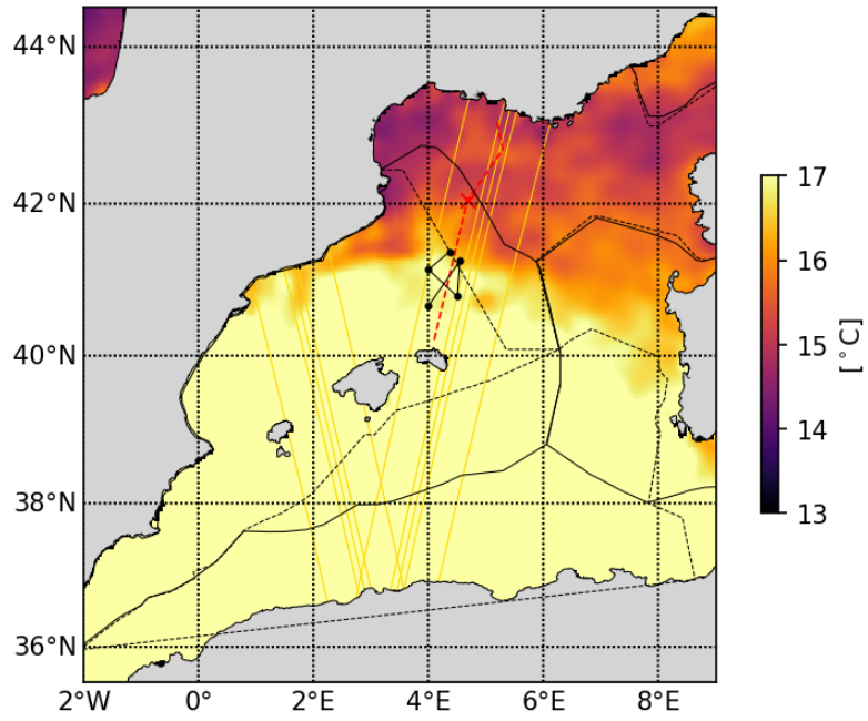
20230426 Tracer advection
