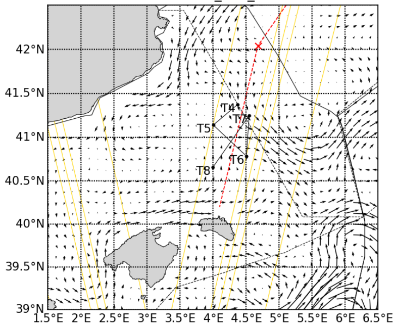
20230420_CLS_PHY
