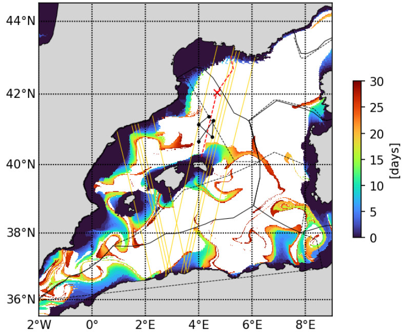
20230426 Timefrombathy_500m
