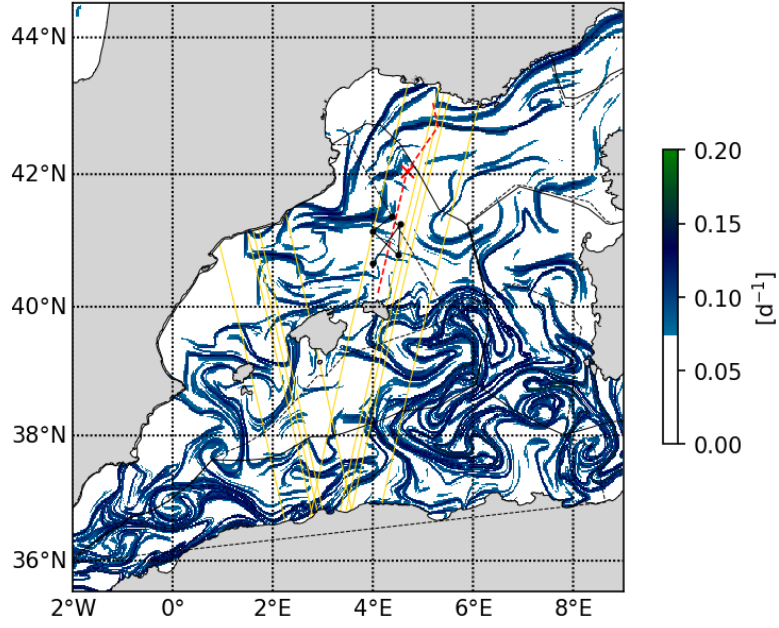
20230426 Finite Time Lyapunov Exponent
