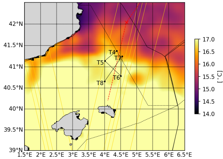
20230426 Tracer advection
