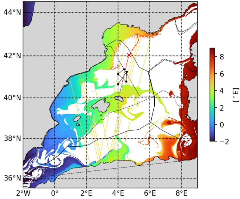
20230426 Lonfrombathy_500m
