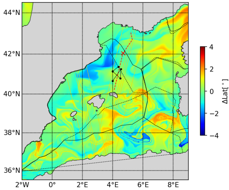
20230426 LatAdv
