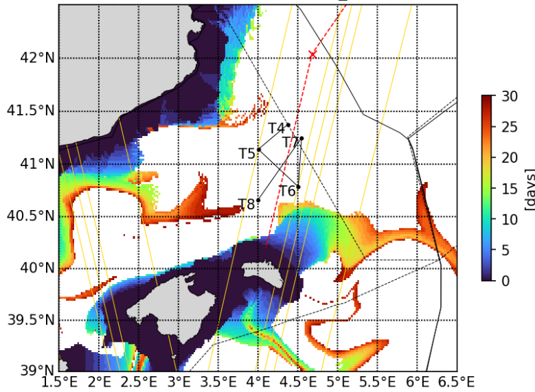
20230426 Timefrombathy_500m
