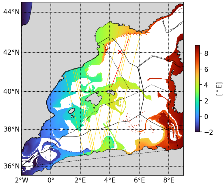
20230417 Lonfrombathy_500m
