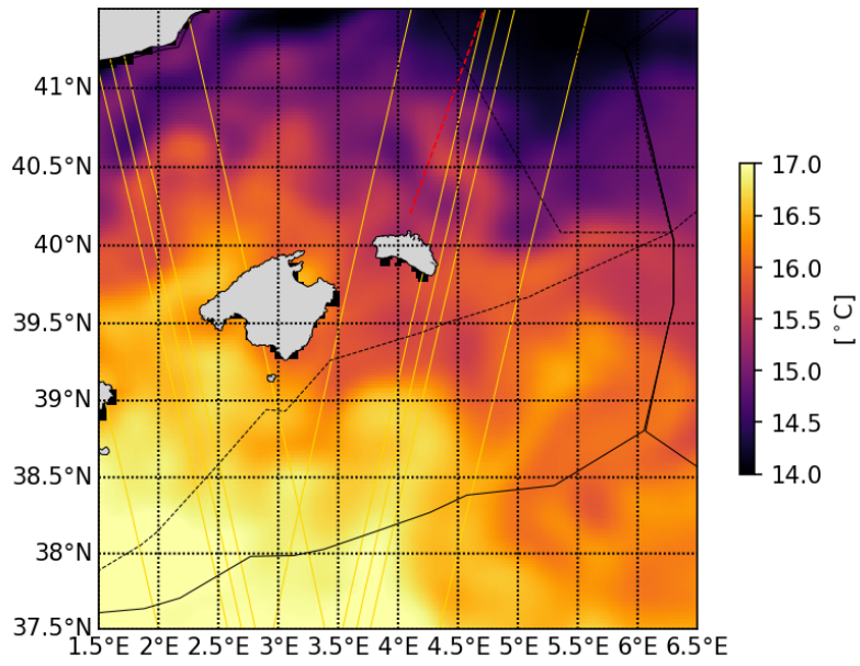
20230417 Tracer advection
