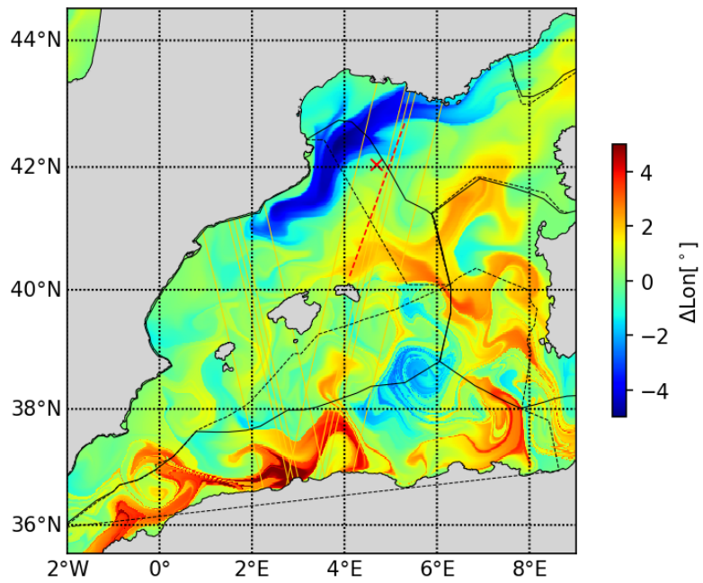
20230417 LonAdv
