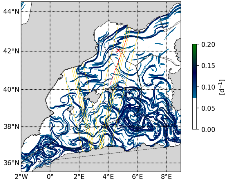
20230417 Finite Time Lyapunov Exponent
