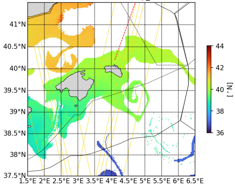
20230417 Latfrombathy_500m
