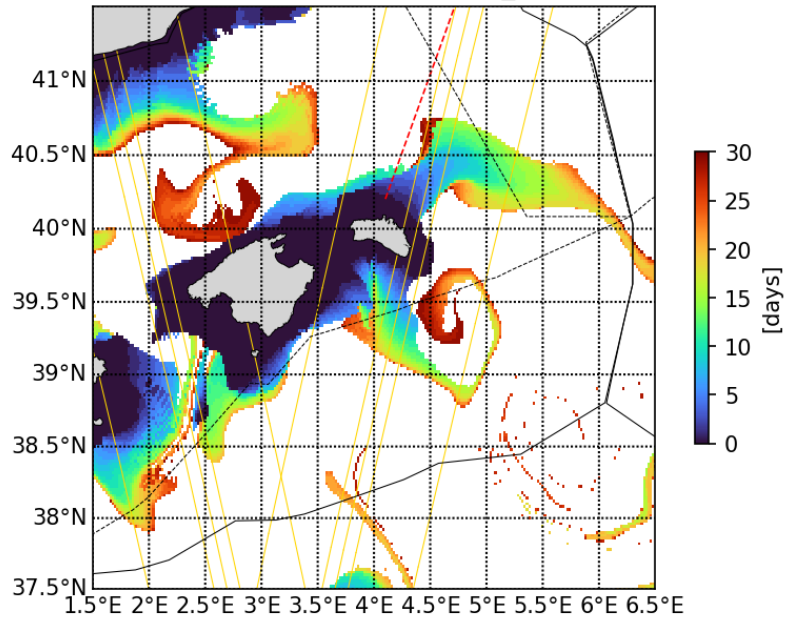
20230417 Timefrombathy_500m
