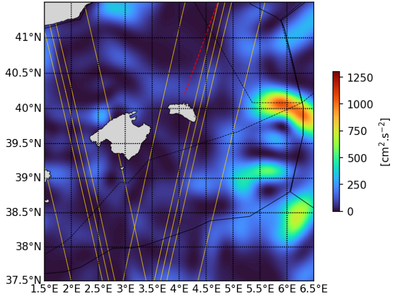
20230417 Kinetic energy
