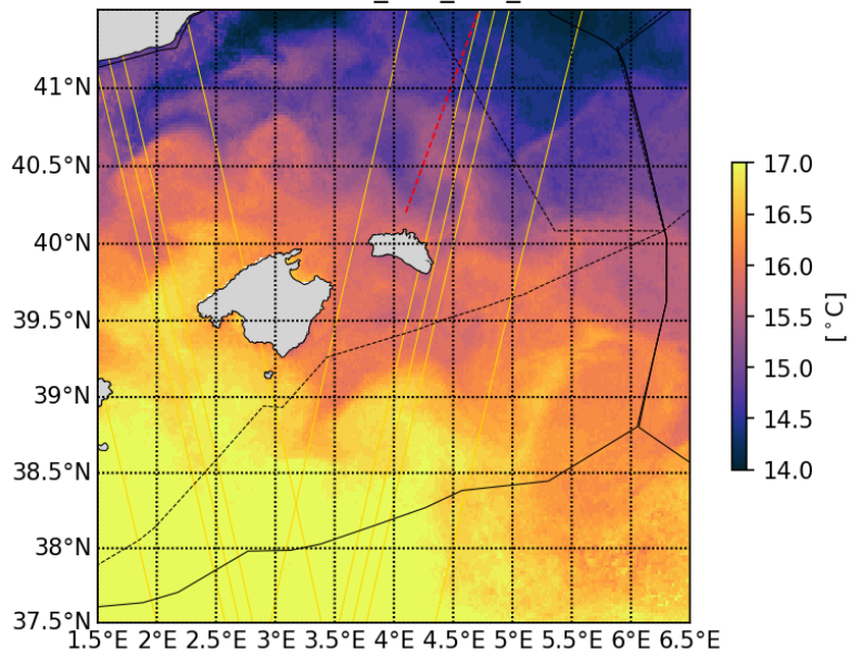
20230415_CLS_SST_5d
