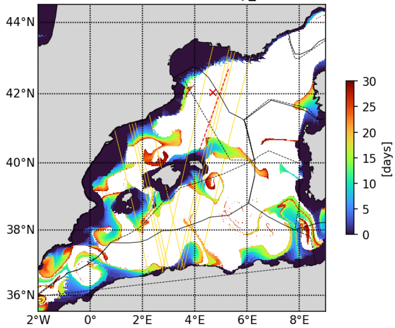
20230417 Timefrombathy_500m
