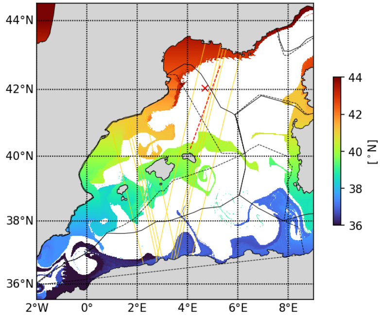
20230417 Latfrombathy_500m
