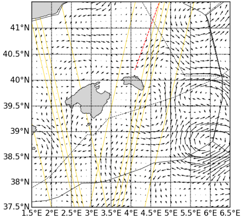
20230411_CLS_PHY
