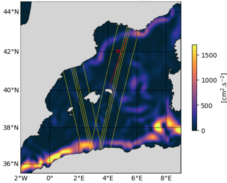
20230312 Kinetic energy
