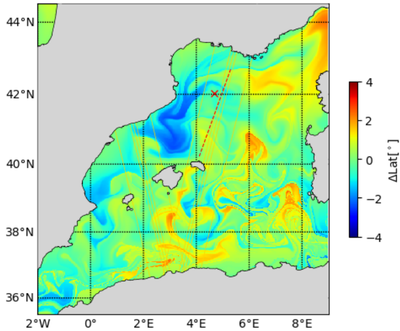
20230312 LatAdv
