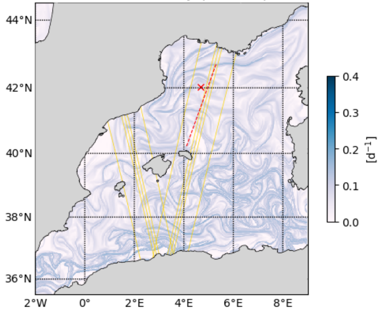
20230312 Finite Time Lyapunov Exponent
