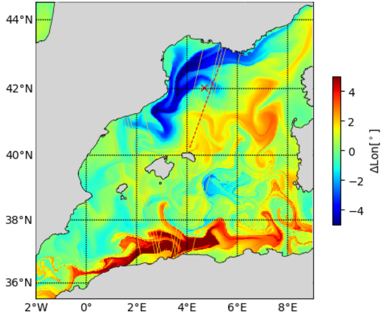
20230312 LonAdv
