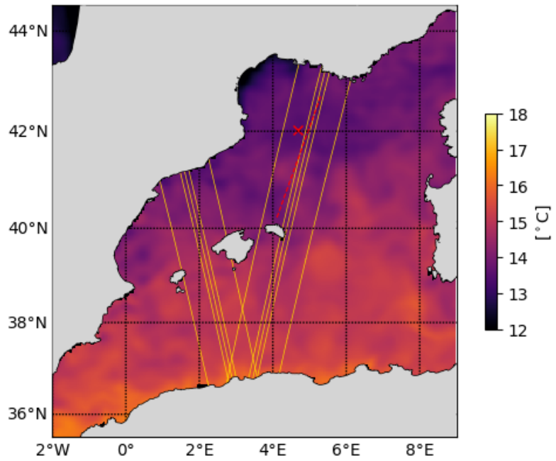
20230312 Tracer advection
