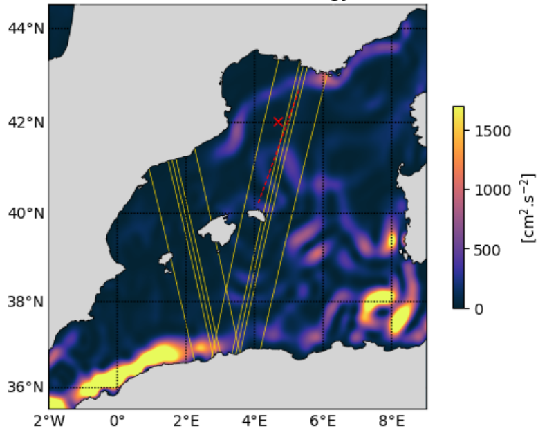
20230302 Kinetic energy
