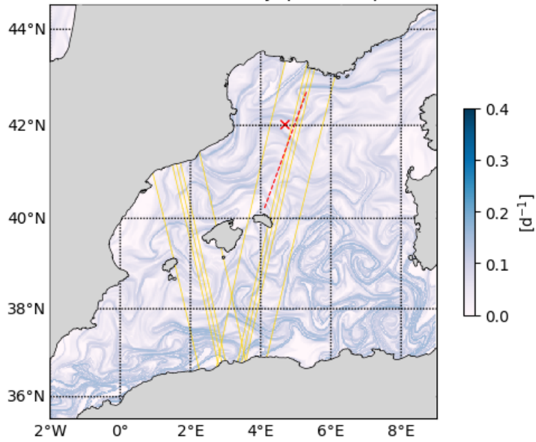
20230302 Finite Time Lyapunov Exponent
